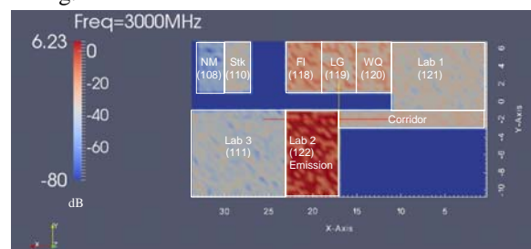
Figure 2. EM cross-coupling between rooms (injection in Lab. 2 room)
