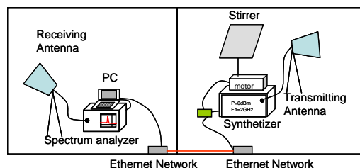
Figure 1. Experimental Set-Up
